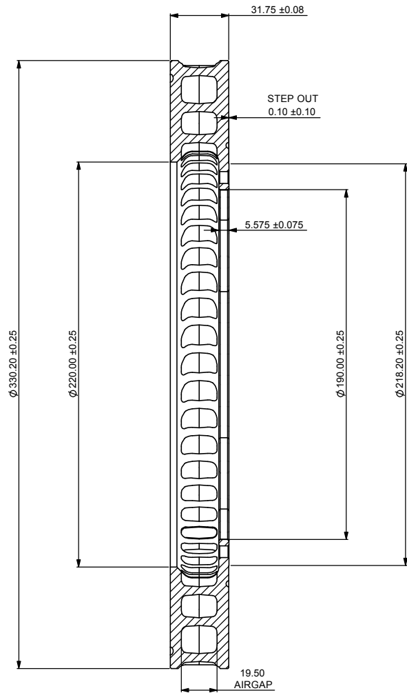
SECTION C-C SCALE 1 : 1
