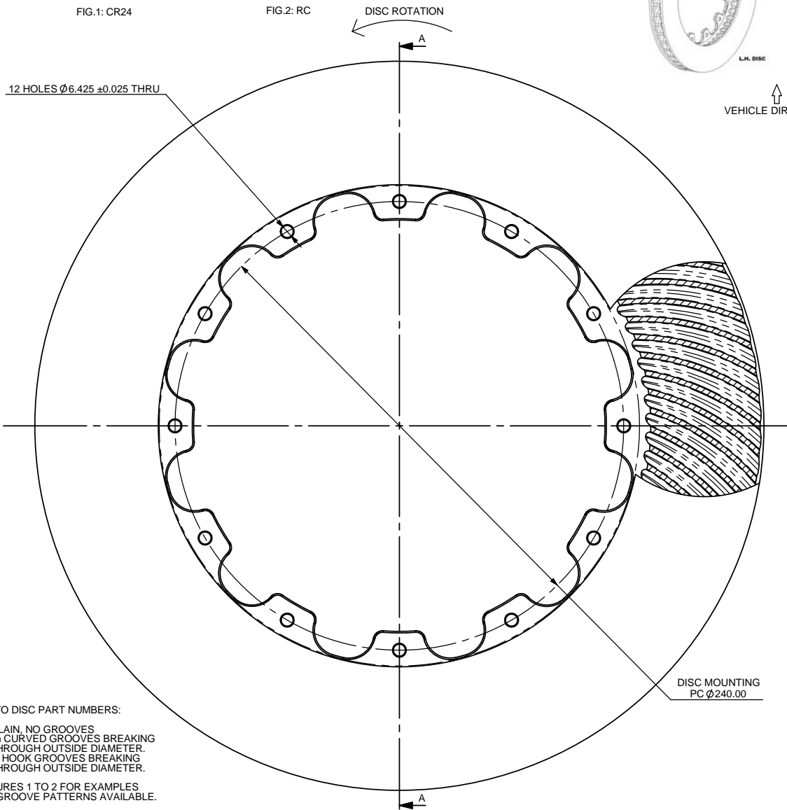
FIG.2: RC
