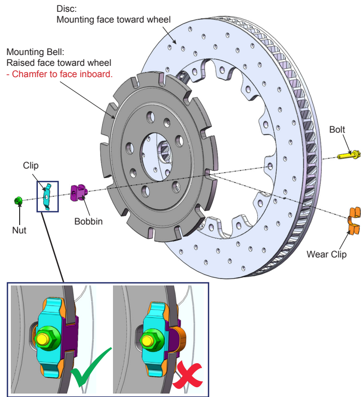
Fig 4. Tighten nut to 6.5Nm
