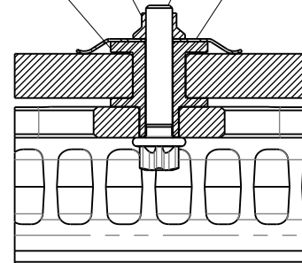
FULL ASSEMBLY SECTION VIEW
